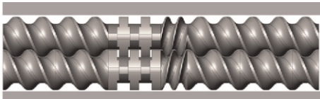
Corotating Twinscrew
