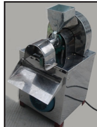
Mini Extruder 50 Kg/Hr for expanded product from corn meal
