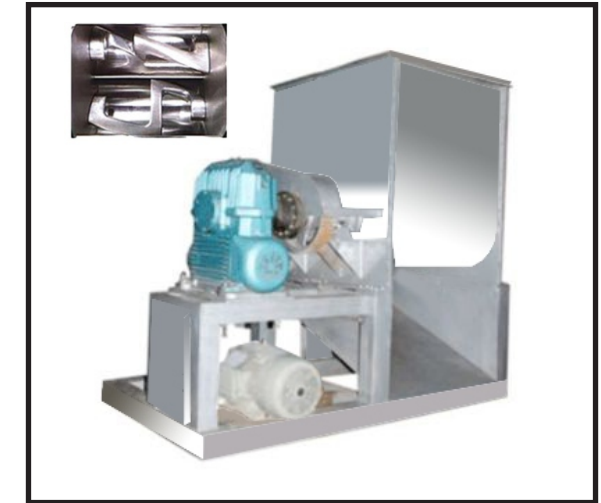
Double Blade Sigma Mixer for Sugar & Gum Base Mixing for Bubble Gum
