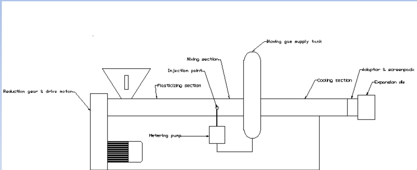
Schematic for Low Density foam (EPE) long barrel extruder
