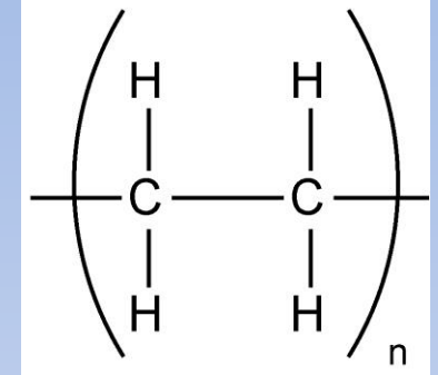
Molecular formula For Polyethylene
